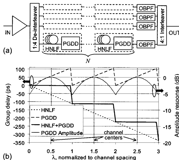
Fig. 1. (a) Schematic of the proposed multichannel dispersion-managed regenerator. In simulations reported in this study, N=16 . (b) Group delay of the HNLF (dotted line), PGDD (dashed curve), and a single HNLF PGDD cell (thick solid curve). Thin solid curve, amplitude transfer function of the PGDD (not considered in 10-Gbit/s simulations).
